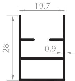
19'LUK PLİSE KASA FRAME PROFILE Kod/Code :SN2021 Ağırlık/Weight :0,244 kg/m
