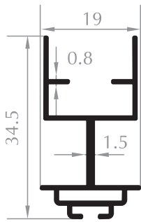
PLİSE KANAT SASH PROFILE Kod/Code :SN2009 Ağırlık/Weight :0,270 kg/m
