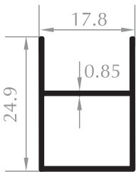
PLİSE KASA FRAME PROFILE Kod/Code :SN2008 Ağırlık/Weight :0,177 kg/m
