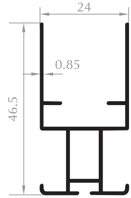
PLİSE KANAT SASH PROFILE Kod/Code :SN2043 Ağırlık/Weight :0,358 kg/m
