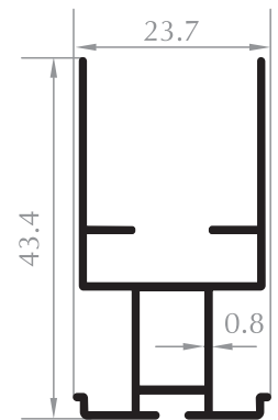
PLİSE KANAT SASH PROFILE Kod/Code :SN2011 Ağırlık/Weight :0,328 kg/m
