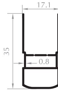
PLİSE KASA FRAME PROFILE Kod/Code :SN2024 Ağırlık/Weight :0,248 kg/m
