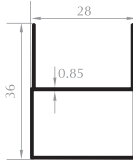
PLİSE KASA FRAME PROFILE Kod/Code :SN2042 Ağırlık/Weight :0,287 kg/m
