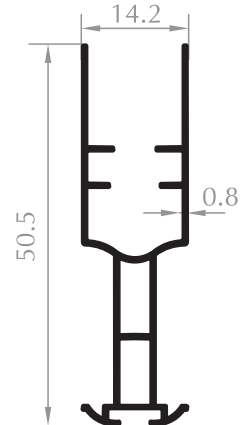
PLİSE KANAT SASH PROFILE Kod/Code :SN2025 Ağırlık/Weight :0,308 kg/m
