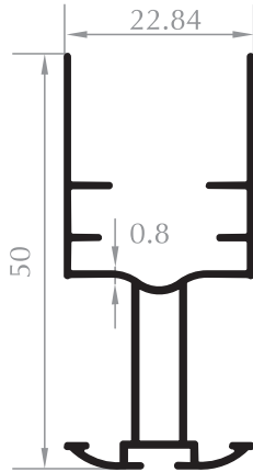
PLİSE KANAT SASH PROFILE Kod/Code :SN2039 Ağırlık/Weight :0,335 kg/m
