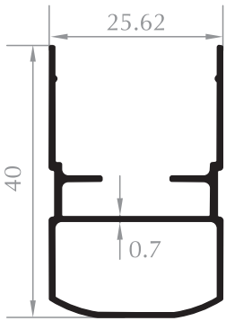
PLİSE KASA FRAME PROFILE Kod/Code :SN2016 Ağırlık/Weight :0,301 kg/m
