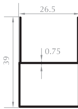
PLİSE KASA FRAME PROFILE Kod/Code :SN2010 Ağırlık/Weight :0,260 kg/m
