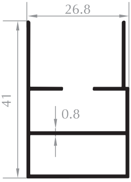
PLİSE KASA FRAME PROFILE Kod/Code :SN2023 Ağırlık/Weight :0,324 kg/m
