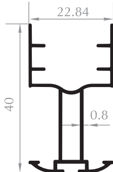
PLİSE KANAT SASH PROFILE Kod/Code :SN2017 Ağırlık/Weight :0,292 kg/m
