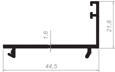
ALÜMİNYUM KAPI ADAPTÖRÜ ADAPTER FOR ALUMINIUM DOOR
