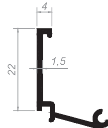
30mm CAM PROFİLİ 30mm GLAZING BEAD Kod/Code :OB-G05 Ağırlık/Weight:0,187 kg/m
