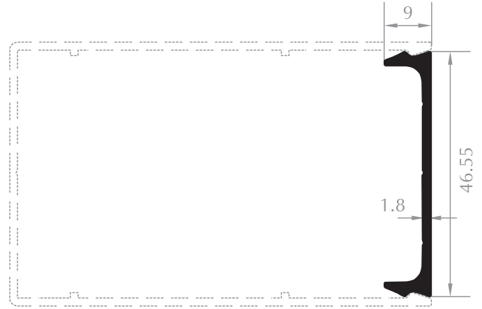
BASKI PROFİLİ COVER PROFILE
