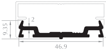
BASKI ÇITASI COVER PROFILE Kod/Code :CE3034 Ağırlık/Weight:0,408 kg/m
