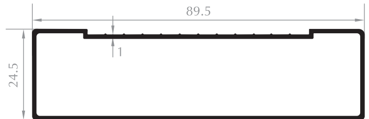
MERDİVEN PROFİLİ STAIRS PROFILE Kod/Code :MH1926 Ağırlık/Weight:0,611 kg/m
