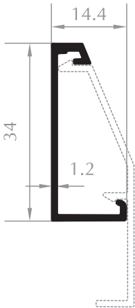
CEPHE PERVAZ PROFİLİ FACADE SILL PROFILE
