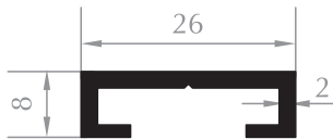
CEPHE PROFİLİ FACADE PROFILE Kod/Code :CE4012 Ağırlık/Weight:0,238 kg/m
