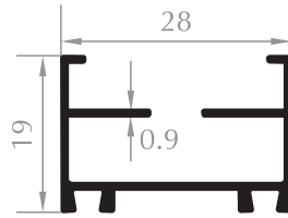
HALATLI FİTİLLİ EKO PROFİLİ VARIOUS PROFILE Kod/Code :MH1105 Ağırlık/Weight:0,250 kg/m
