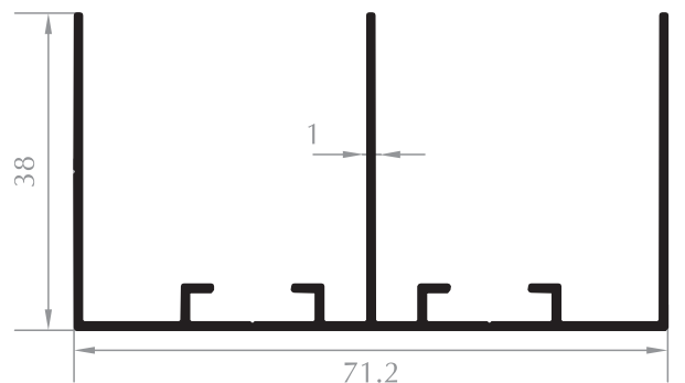
MOBİLYA PROFİLİ FURNITURE PROFILE Kod/Code :MB1019 Ağırlık/Weight:0,572 kg/m
