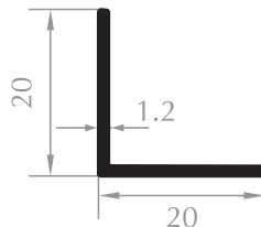
L PROFİL L PROFILE
