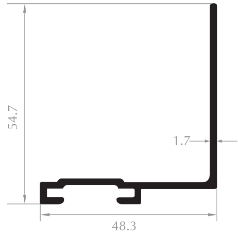
TEK KANALLI L PROFİL SINGLE CHANNEL L PROFILE Kod/Code :CE1605 Ağırlık/Weight:0,530 kg/m
