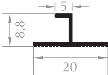
10'LUK DİKEY DERZ PROFİLİ VERTICAL JOINT PROFILE
