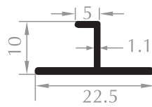
YATAY DERZ PROFİLİ HORIZONTAL JOINT PROFILE
