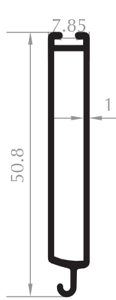
ALT ETEK PROFİLİ LOWER PROFILE Kod/Code :PJ1003 Ağırlık/Weight:0,312 kg/m
