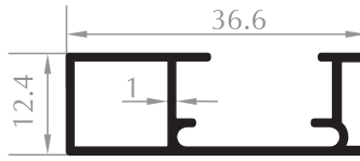
İÇ RAY INNER RAIL PROFILE Kod/Code :DK1002 Ağırlık/Weight:0,244 kg/m
