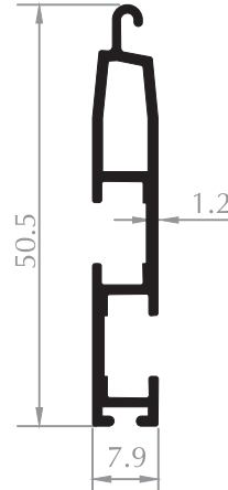
PANJUR PROFİLİ SHUTTER PROFILE Kod/Code :PJ1031 Ağırlık/Weight:0,358 kg/m
