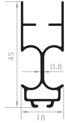
PLİSE KANAT SASH PROFILE Kod/Code : SN2038 Ağırlık/Weight : 0,329 kg/m
