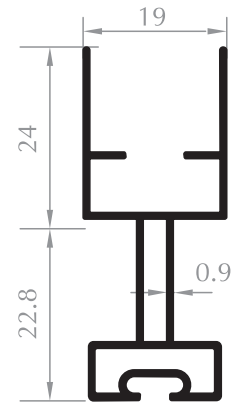
19'LUK PLİSE KANAT SASH PROFILE Kod/Code :SN2022 Ağırlık/Weight :0,394 kg/m
