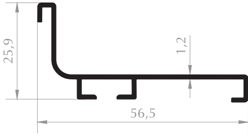
MUTFAK TEZGAH PROFİLİ KITCHEN COUNTER PROFILE Kod/Code : MB3014 Ağırlık/Weight : 0,342 kg/m
