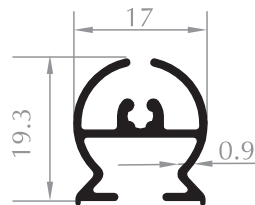
ORTA DİKME MIDDLE PROFILE Kod/Code :DK1011 Ağırlık/Weight:0,214 kg/m
