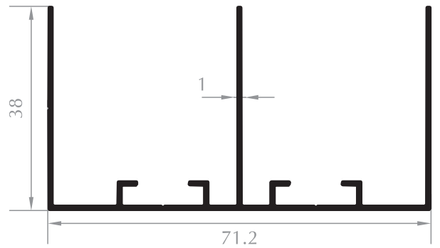
MOBİLYA PROFİLİ FURNITURE PROFILE Kod/Code :MB1019 Ağırlık/Weight:0,572 kg/m
