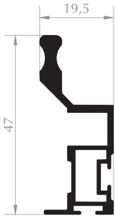
SÜRGÜ DOLAP PROFİLİ SLIDING WARDROBE PROFILE Kod/Code :MB1058 Ağırlık/Weight:0,547 kg/m
