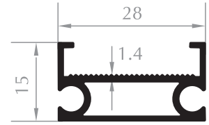
ZEMİN PROFİLİ FLOORING PROFILE Kod/Code :MH1103 Ağırlık/Weight:0,303 kg/m
