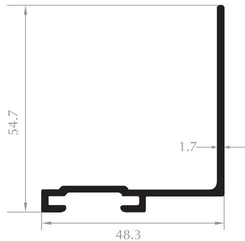
TEK KANALLI L PROFİL SINGLE CHANNEL L PROFILE Kod/Code : CE1605 Ağırlık/Weight: 0,530 kg/m
