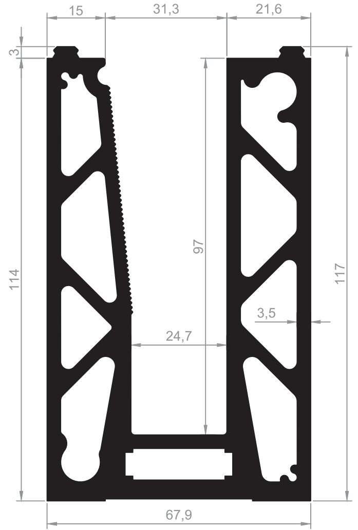
ALT BAZA PROFİLİ BASE PROFILE
