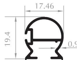
ARKA DİKME VERTICAL BACK PROFILE Kod/Code :DK1012 Ağırlık/Weight:0,202 kg/m
