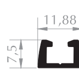
MOBİLYA PROFİLİ FURNITURE PROFILE Kod/Code : MB3006 Ağırlık/Weight : 0,114 kg/m
