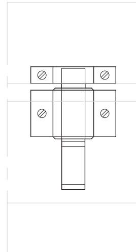
DH-06 VASİSTAS KİLİDİ FINGER CATCHER FOR VASİSTAS WINDOW
