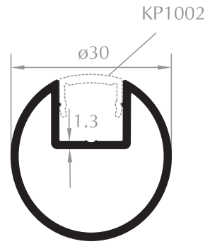
30'LUK KANALLI BORU Ø30 SINGLE CHANNEL PIPE Kod/Code : KP1034 Ağırlık/Weight : 0,389 kg/m
