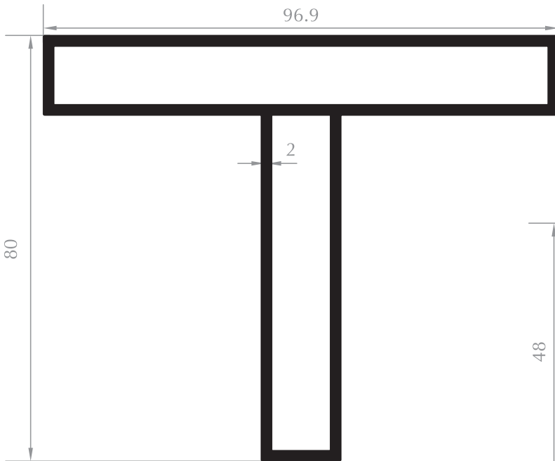
T PROFİL T PROFILE Kod/Code :CE4026 Ağırlık/Weight: 1,933 kg/m
