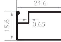
17x25 PENCERE SİNEKLİK 17x25 FLYSCREEN FOR WINDOW Kod/Code : SN1002 Ağırlık/Weight : 0,153 kg/m
