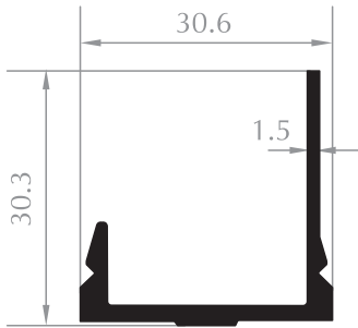
BASKI PROFİLİ COVER PROFILE Kod/Code :CE4008 Ağırlık/Weight:0,336 kg/m
