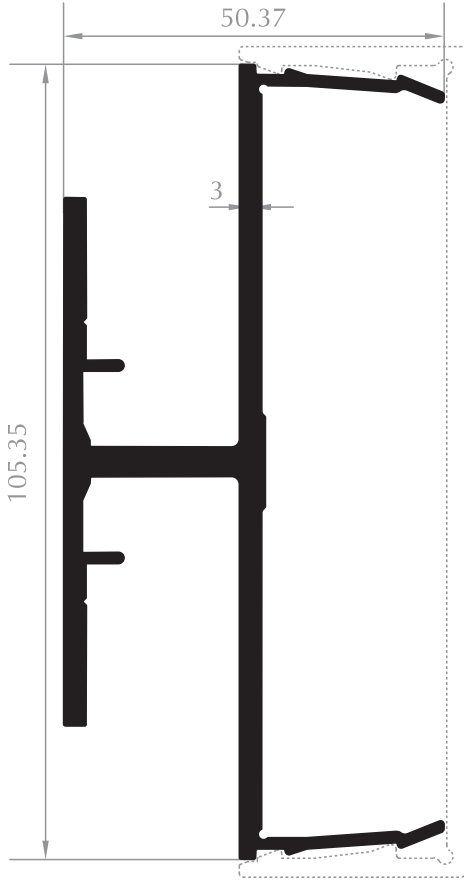
BASKI PROFİLİ COVER PROFILE Kod/Code :CE4024 Ağırlık/Weight: 1,884 kg/m
