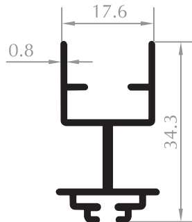
PLİSE KANAT SASH PROFILE Kod/Code :SN2053 Ağırlık/Weight :0,261 kg/m
