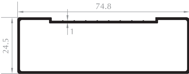
MERDİVEN PROFİLİ STAIRS PROFILE Kod/Code :MH1925 Ağırlık/Weight:0,531 kg/m
