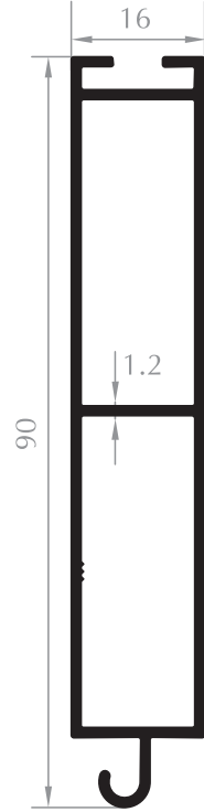
ALT ETEK PROFİL LOWER PROFILE Kod/Code :PJ1005 Ağırlık/Weight:0,735 kg/m
