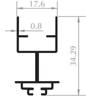
PLİSE KANAT SASH PROFILE Kod/Code :SN-2053 Ağırlık/Weight :0,261 kg/m
