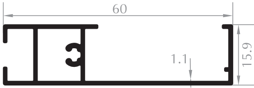
DİŞ RAY OUTER RAIL PROFILE Kod/Code :DK1001 Ağırlık/Weight:0,444 kg/m
