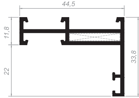
KASA PROFİLİ FRAME PROFILE
