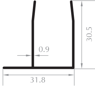
DUVAR DİKMEĐ VERTICAL WALL PROFILE Kod/Code :DK4004 Ağırlık/Weight:0,221 kg/m
