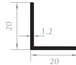
L PROFİL L PROFILE
