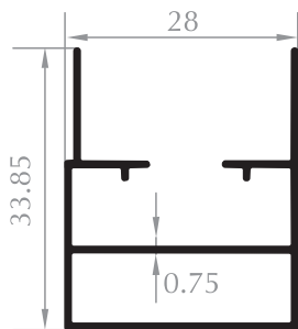
PLİSE KASA FRAME PROFILE Kod/Code :SN2013 Ağırlık/Weight :0,287 kg/m
