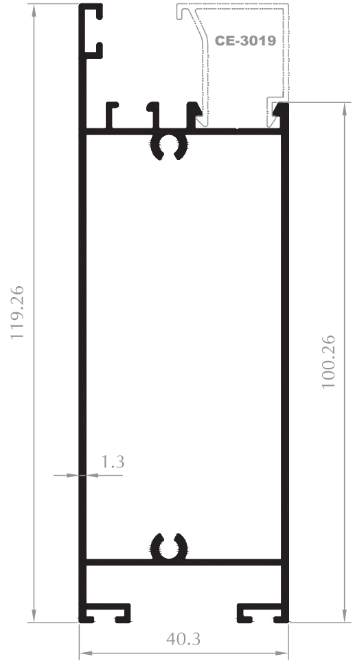
ETEK PROFİLİ KICK PLATE PROFILE Kod/Code : CE3021 Ağırlık/Weight: 1,254 kg/m
