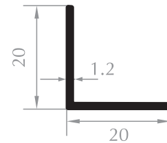
L PROFİL L PROFILE Kod/Code :ST2006 Ağırlık/Weight:0,126 kg/m
