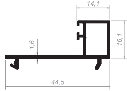
CAM KAPI ADAPTÖRÜ ADAPTER FOR GLASS DOOR
