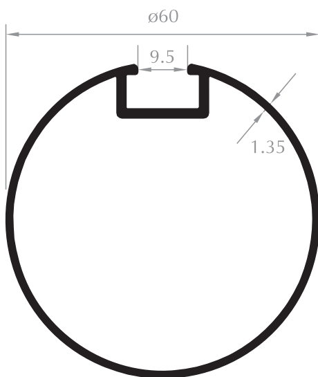
OTOMOTİV BORU PROFİLİ AUTOMATIVE PROFILE Kod/Code :MH1955 Ağırlık/Weight:0,793 kg/m
