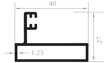
YAN DİKME SIDE VERTICAL Kod/Code :CB2003 Ağırlık/Weight :0,447 kg/m
