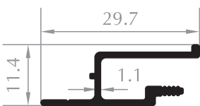
GERGİ TAVAN PROFİLİ CEILING PROFILE Kod/Code :MH1916 Ağırlık/Weight:0,188 kg/m
