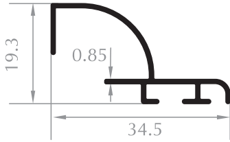
MENFEZ KASA VENT FRAME
