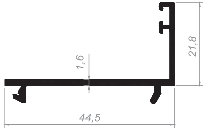
ALÜMİNYUM KAPI ADAPTÖRÜ ADAPTER FOR ALUMINIUM DOOR
