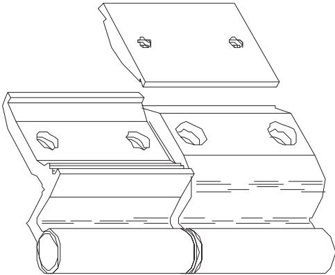
DH-03 180° AÇILABİLEN MENTEŞE REVERSIBLE HINGE WITH COUPLING PLATE OPENING 180°
