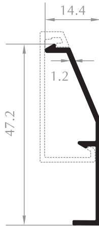
CEPHE PERVAZ PROFİLİ FACADE SILL PROFILE Kod/Code :CE4020 Ağırlık/Weight:0,211 kg/m
