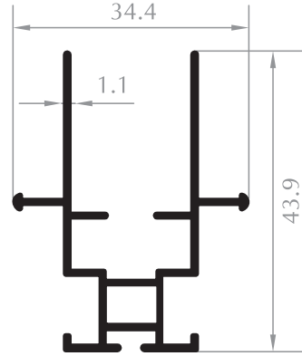
PLİSE KANAT SASH PROFILE Kod/Code :SN2003 Ağırlık/Weight :0,370 kg/m
