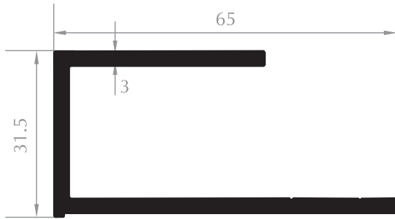
ALT U PROFİL BOTTOM U PROFILE Kod/Code : KP1006 Ağırlık/Weight : 1,064 kg/m
