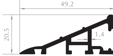
ZEMİN PROFİLİ FLOORING PROFILE Kod/Code :MH1102 Ağırlık/Weight:0,575 kg/m
