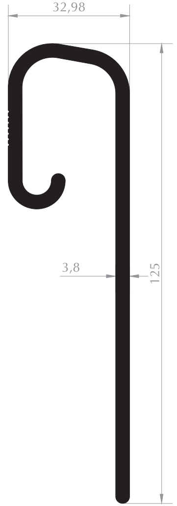
MOBİLYA PROFİLİ FURNITURE PROFILE Kod/Code :MB1037 Ağırlık/Weight:2,032 kg/m
