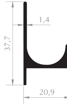
MOBİLYA PROFİLİ FURNITURE PROFILE Kod/Code : MB3020 Ağırlık/Weight : 0,357 kg/m
