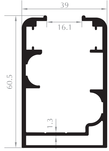
CAM BALKON KASA FRAME PROFILE Kod/Code :CB2006 Ağırlık/Weight :1,131 kg/m
