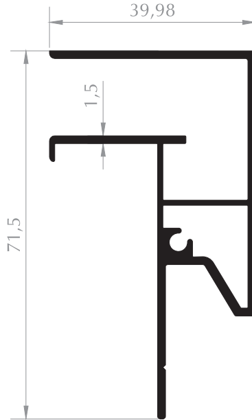
MOBİLYA PROFİLİ FURNITURE PROFILE Kod/Code : MB3030 Ağırlık/Weight: 0,840 kg/m
