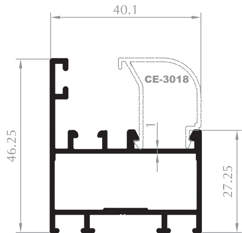
KASA PROFİLİ FRAME PROFILE
