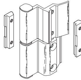
DH-04 180° AÇILIR İTHAL İKİNCİ KANAT MENTEŞE REVERSIBLE HINGE WITH COUPLING PLATE OPENING 180°
