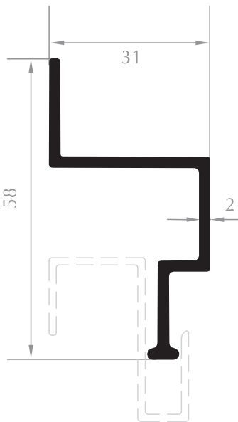
ASKI PROFİLİ HANGER PROFILE Kod/Code :CE2502 Ağırlık/Weight:0,536 kg/m
