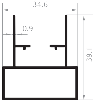
PLİSE KASA FRAME PROFILE Kod/Code :SN2004 Ağırlık/Weight :0,367 kg/m
