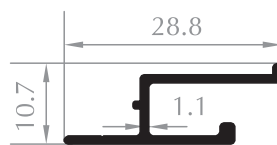
GERGİ TAVAN PROFİLİ CEILING PROFILE Kod/Code :MH1917 Ağırlık/Weight:0,160 kg/m
