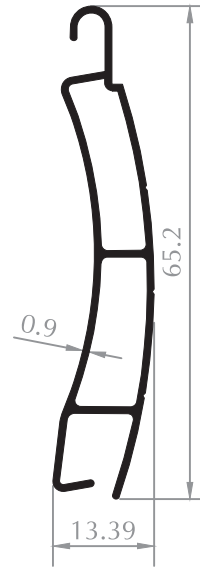
PANJUR PROFİLİ SHUTTER PROFILE Kod/Code :PJ1030 Ağırlık/Weight:0,374 kg/m
