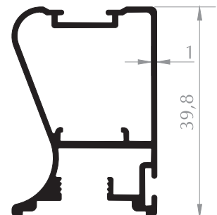
RAY KAPAK PROFİLİ RAIL PROFILE Kod/Code : MB1057 Ağırlık/Weight : 0,488 kg/m
