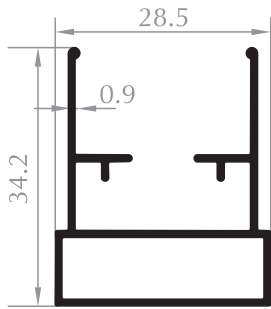
PLİSE KASA FRAME PROFILE Kod/Code :SN2005 Ağırlık/Weight :0,349 kg/m
