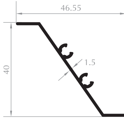
MENFEZ Z PROFİLİ VENT Z PROFILE
