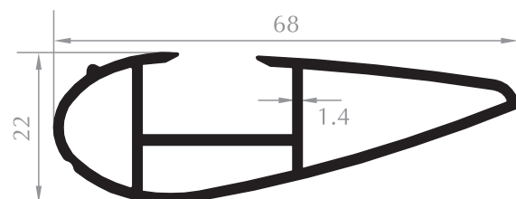
68'LİK OTOMOTİV PROFİLİ AUTOMATIVE PROFILE Kod/Code : MH1954 Ağırlık/Weight : 0,728 kg/m
