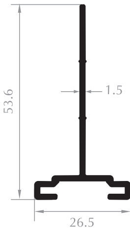
TEK KANALLI T SINGLE CHANNEL T PROFILE Kod/Code : CE1601 Ağırlık/Weight: 0,375 kg/m
