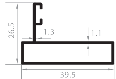
YAN DİKME SIDE VERTICAL Kod/Code :CB2008 Ağırlık/Weight :0,344 kg/m
