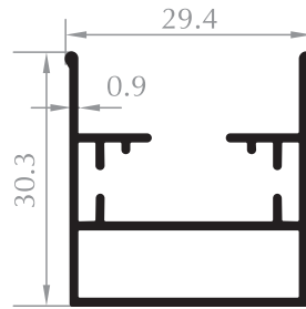
PLİSE KASA FRAME PROFILE Kod/Code :SN2006 Ağırlık/Weight :0,368 kg/m
