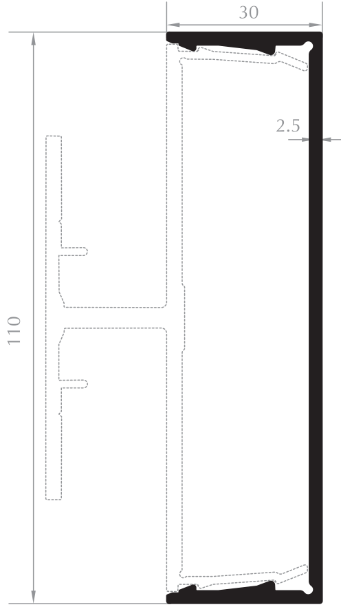
KAPAK PROFİLİ CAP PROFILE Kod/Code :CE4025 Ağırlık/Weight: 1,155 kg/m
