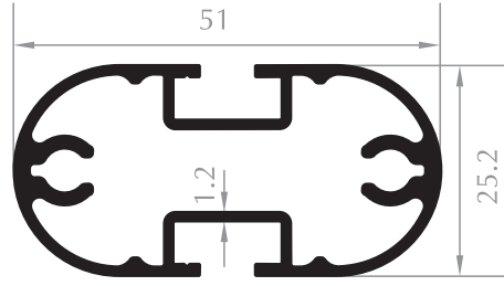
KANALLI ELİPS BORU PIPE PROFILE WITH CHANNEL Kod/Code :RK1002 Ağırlık/Weight:0,749 kg/m
