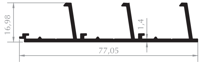
MENFEZ PROFİLİ VENT PROFILE
