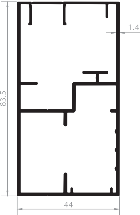
PANJUR PROFİLİ SHUTTER PROFILE Kod/Code :PJ1028 Ağırlık/Weight:1,333 kg/m
