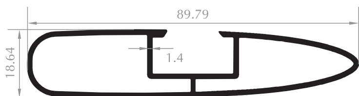
90°'LİK OTOMOTİV PROFİLİ AUTOMATIVE PROFILE Kod/Code :MH1956 Ağırlık/Weight:0,859 kg/m
