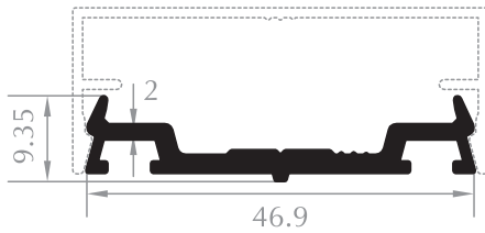
BASKI ÇITASI COVER PROFILE
