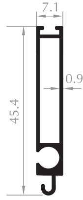
ALT ETEK PROFİLİ LOWER PROFILE Kod/Code :PJ1021 Ağırlık/Weight:0,262 kg/m
