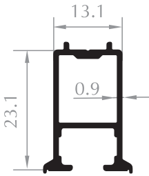
ARKA SABİT BACK FIXING PROFILE Kod/Code :DK1007 Ağırlık/Weight:0,224 kg/m
