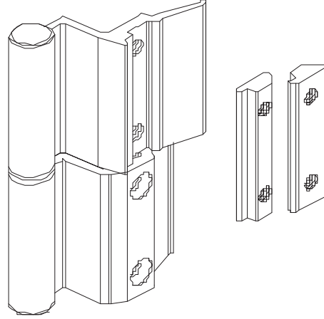
DH-02 180° AÇILABİLEN MENTEŞE REVERSIBLE HINGE WITH COUPLING PLATE OPENING 180°
