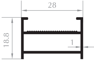
ZEMİN PROFİLİ FLOORING PROFILE Kod/Code :MH1101 Ağırlık/Weight:0,268 kg/m
