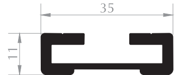
MOBİLYA PROFİLİ FURNITURE PROFILE Kod/Code :MB1038 Ağırlık/Weight:0,470 kg/m
