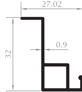
SİNEKLİK PROFİLİ FLYSCREEN PROFILE Kod/Code :SN2051 Ağırlık/Weight :0,206 kg/m
