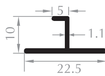
YATAY DERZ PROFİLİ HORIZONTAL JOINT PROFILE Kod/Code : CE1410 Ağırlık/Weight : 0,103 kg/m
