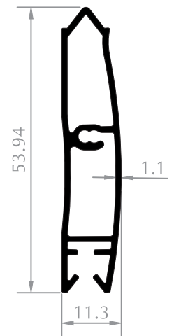
PANJUR PROFİLİ SHUTTER PROFILE Kod/Code :PJ1029 Ağırlık/Weight:0,436 kg/m
