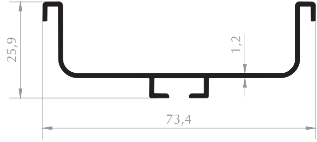
MUTFAK TEZGAH PROFİLİ KITCHEN COUNTER PROFILE Kod/Code : MB3015 Ağırlık/Weight : 0,434 kg/m
