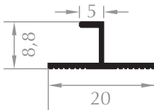
10'LUK DİKEY DERZ PROFİLİ VERTICAL JOINT PROFILE Kod/Code : CE1411 Ağırlık/Weight : 0,081 kg/m
