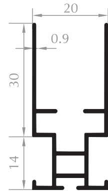
PLİSE KANAT SASH PROFILE Kod/Code :SN2007 Ağırlık/Weight :0,348 kg/m
