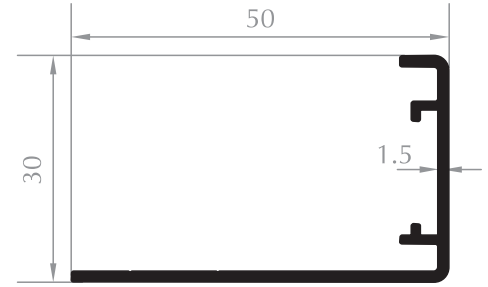
PERVAZ PROFİLİ SILL PROFILE Kod/Code :CE4040 Ağırlık/Weight:0,372 kg/m
