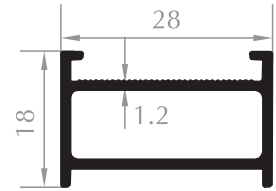
ZEMİN PROFİLİ FLOORING PROFILE Kod/Code :MH1106 Ağırlık/Weight:0,324 kg/m
