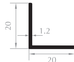
L PROFİL L PROFILE Kod/Code :ST2006 Ağırlık/Weight:0,126 kg/m
