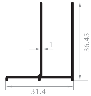
DUVAR DİKME VERTICAL WALL PROFILE Kod/Code :DK1004 Ağırlık/Weight:0,280 kg/m
