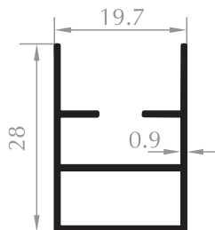
19'LUK PLİSE KASA FRAME PROFILE Kod/Code :SN2021 Ağırlık/Weight :0,244 kg/m
