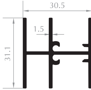
MOBİLYA PROFİLİ FURNITURE PROFILE Kod/Code :MB1005 Ağırlık/Weight:0,518 kg/m
