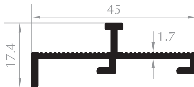
ARA ASKI PROFİLİ HANGER PROFILE Kod/Code : CE1903 Ağırlık/Weight : 0,351 kg/m
