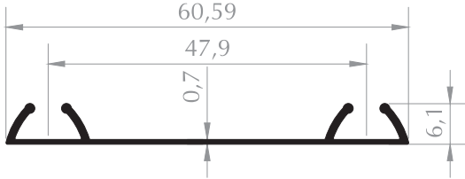
ALT RAY PROFİLİ RAIL PROFILE Kod/Code : MB1026 Ağırlık/Weight : 0,193 kg/m
