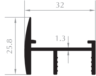
MOBİLYA PROFİLİ FURNITURE PROFILE Kod/Code :MB1006 Ağırlık/Weight:0,386 kg/m
