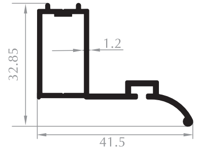
KISA KAPI KARŞILIK ADAPTER FOR DOOR SASH Kod/Code :DK1013 Ağırlık/Weight:0,406 kg/m
