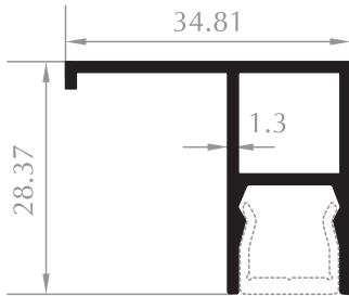
DERZ PROFİLİ JOINT PROFILE Kod/Code :MH1970 Ağırlık/Weight:0,381 kg/m
