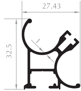
KÖŞE DİKME VERTICAL CORNER PROFILE Kod/Code :DK1009 Ağırlık/Weight:0,418 kg/m
