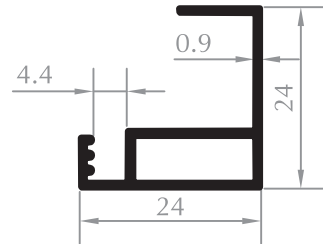
SİNEKLİK PROFİLİ FLYSCREEN PROFILE Kod/Code :SN2054 Ağırlık/Weight :0,221 kg/m
