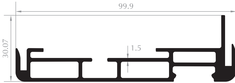
SOĞUTMA PROFİLİ REFRIGERATION PROFILE Kod/Code :MH1961 Ağırlık/Weight: 1,377 kg/m
