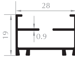
HALATLI FİTİLLİ EKO PROFİLİ VARIOUS PROFILE Kod/Code :MH1105 Ağırlık/Weight:0,250 kg/m
