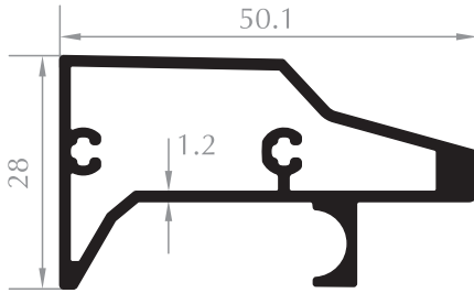
RAY PROFİLİ RAIL PROFILE Kod/Code :DK4103 Ağırlık/Weight:0,638 kg/m
