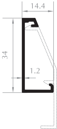
CEPHE PERVAZ PROFİLİ FACADE SILL PROFILE Kod/Code :CE4019 Ağırlık/Weight:0,201 kg/m
