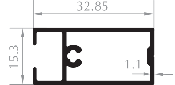
ASKILIK HANGER PROFILE Kod/Code :DK1006 Ağırlık/Weight:0,332 kg/m
