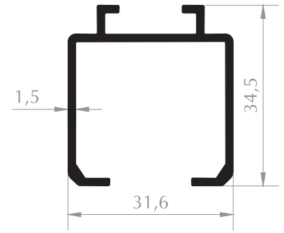
MOBİLYA PROFİLİ FURNITURE PROFILE Kod/Code :MB1031 Ağırlık/Weight:0,473 kg/m
