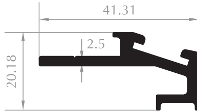
CEPHE PROFİLİ FACADE PROFILE Kod/Code :CE4013 Ağırlık/Weight:0,529 kg/m
