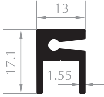
MOBİLYA PROFİLİ FURNITURE PROFILE Kod/Code :MB1004 Ağırlık/Weight:0,296 kg/m
