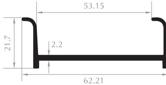
ASKI PROFİLİ HANGER PROFILE Kod/Code :CE1103 Ağırlık/Weight:0,582 kg/m
