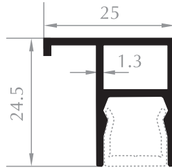
DERZ PROFİLİ JOINT PROFILE Kod/Code :CE4038 Ağırlık/Weight:0,320 kg/m
