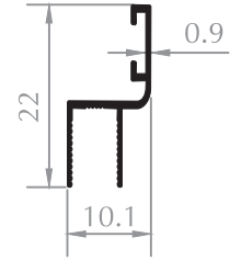
CAM PROFİLİ GLASS PROFILE Kod/Code :CB3013 Ağırlık/Weight: 0,125 kg/m
