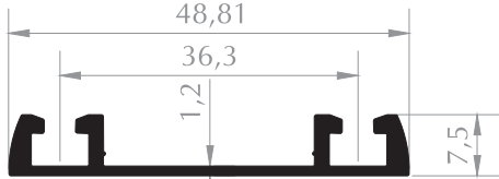
ALT RAY PROFİLİ RAIL PROFILE Kod/Code : MB3001 Ağırlık/Weight : 0,330 kg/m
